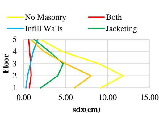
Fig. 1. Graphe of Story drift "sdx" of each floor for the 4 models (without retrofitting, with jacketing, with infill walls, with both), obtained by the THA on STERA-3D using the record of Boumerdes 2003 Eq.
